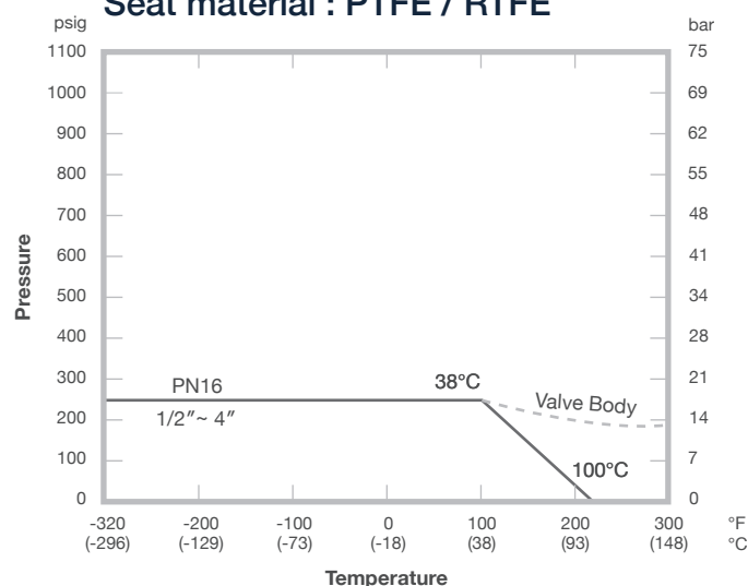
Series F520-40 Seat material : PTFE / RTFE
