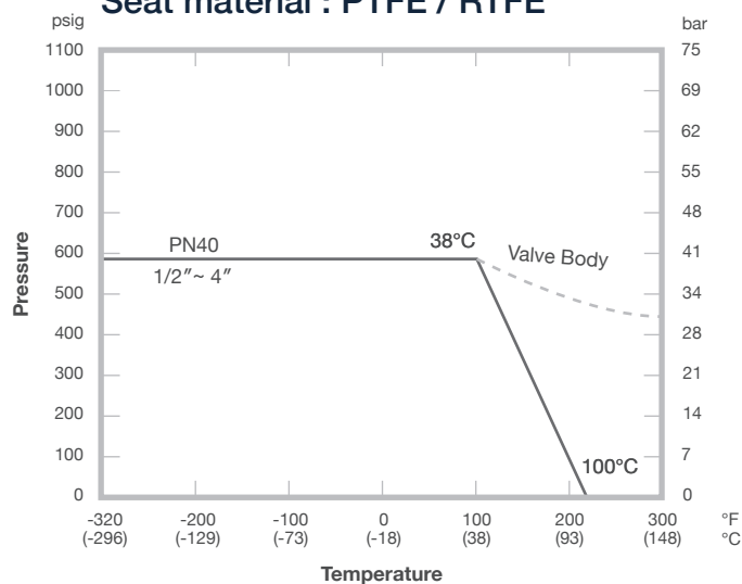
Series F520-60 Seat material : PTFE / RTFE
